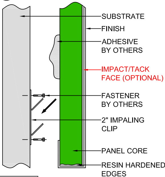
1 ATTACHMENT DETAIL CX-01 SCALE: NA
