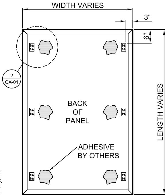
A IMPALING CLIP ATTACHMENT CX-02 SCALE: NA
